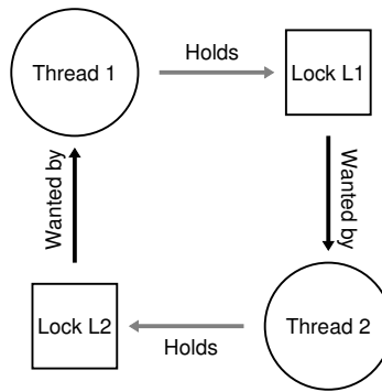
Figure 32.7: The Deadlock Dependency Graph
